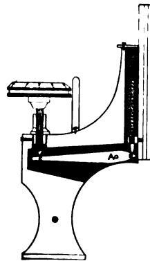
FIG. 43.—Fine adjustment.
